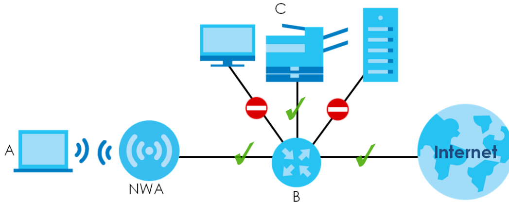
Figure 82 Layer-2 Isolation Application
