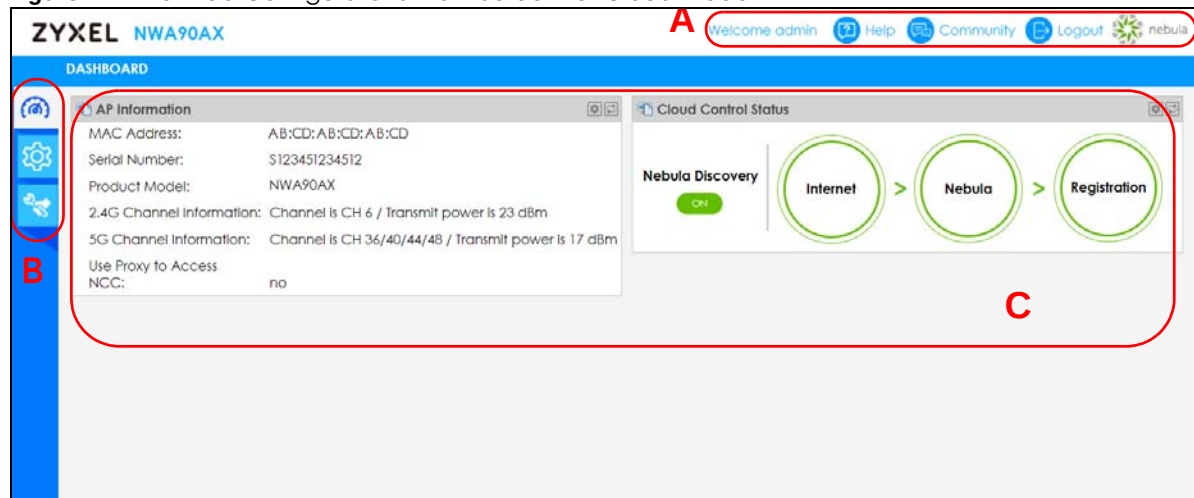
Figure 21 The Web Configurator's Main Screen for Cloud Mode
