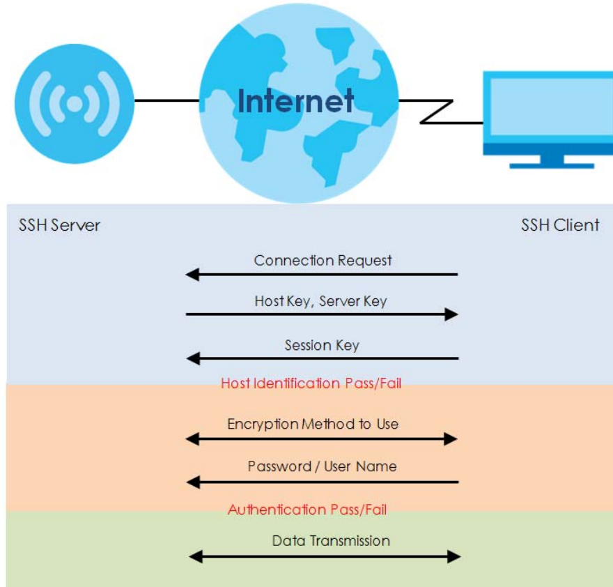
Figure 104 How SSH v1 Works Example
