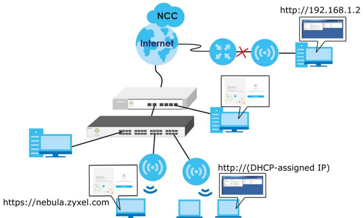
Figure 124 Cloud Mode Application
